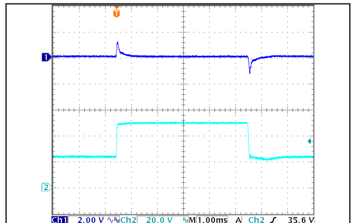
Figure 6: Output voltage response to step-change in input voltage (500 V/ms). Load cap: 100 \mu F , electrolytic output capacitance. Ch 1: V_{out} (2 V/div), Ch 2: V_{in} (20 V/div).
