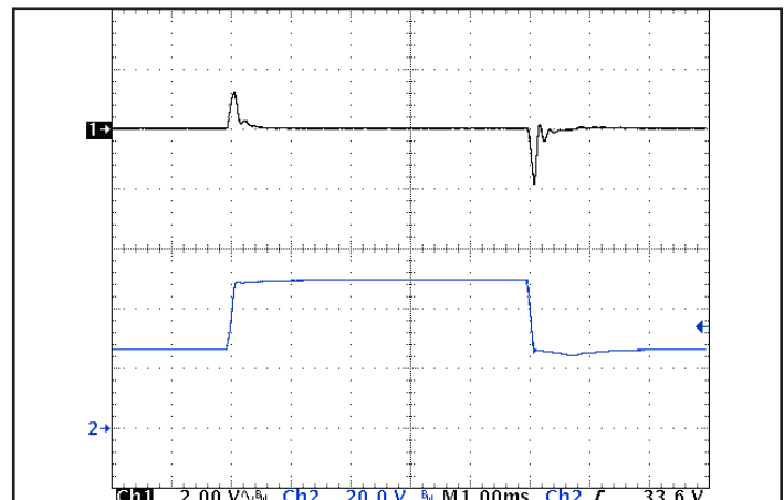
Figure 6: Output voltage response to step-change in input voltage (500 V/ms). Load cap: 100 μF, electrolytic output capacitance. Ch 1: V out (2 V/div), Ch 2: V in (20 V/div).
