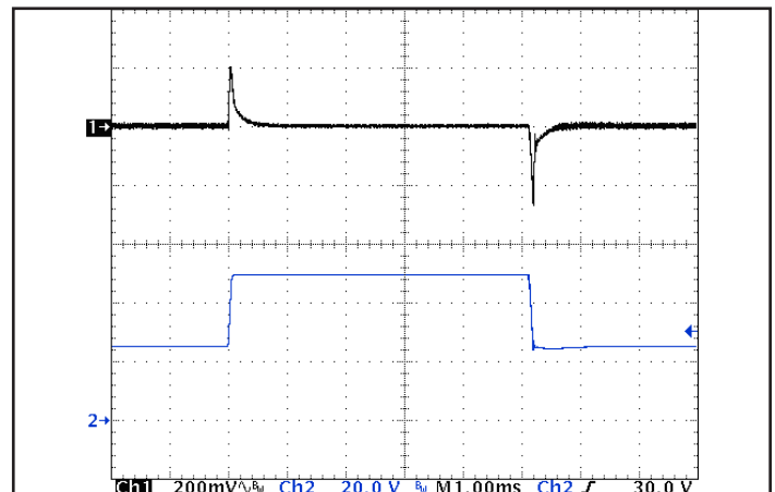
Figure 6: Output voltage response to step-change in input voltage (500 V/ms). Load cap: 100 \mu F , electrolytic output capacitance. Ch 1: V_{out} (200 mV/div), Ch 2: V_{in} (20 V/div).
