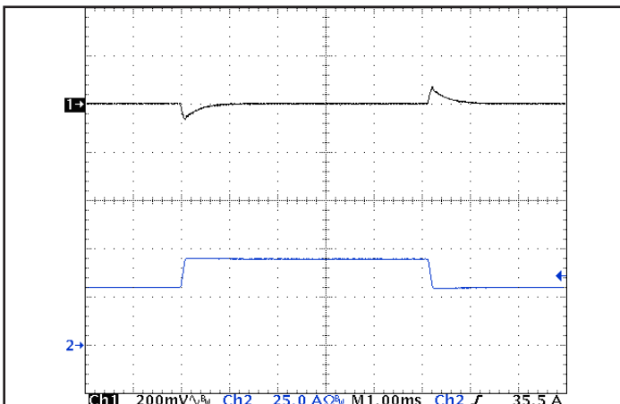
Figure 5: Output voltage response to step-change in load current (66 %-100 %-66 % of I out (max); dI/dt = 0.2 A/μs). Load cap: 1 μF ceramic and 15 μF tantalum capacitors. Ch 1: V out (200 mV/div), Ch 2: I out (25 A/div).
