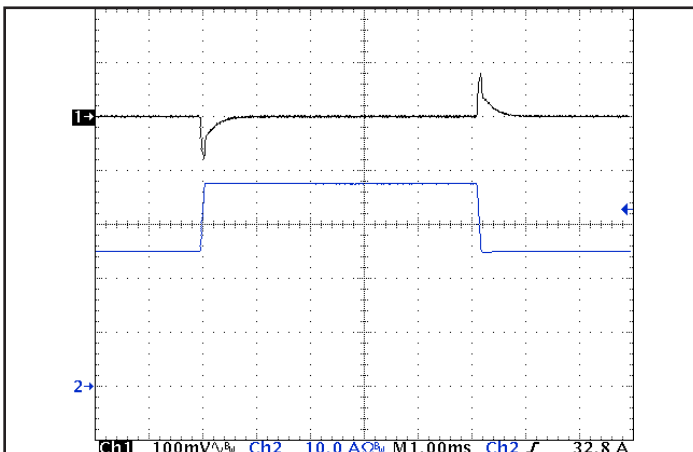
Figure 5: Output voltage response to step-change in load current (66 %-100 %-66 % of I out (max); dI/dt = 0.2 A/μs). Load cap: 1 μF ceramic and 15 μF tantalum capacitors. Ch 1: V out (100 mV/div), Ch 2: I out (10 A/div).
