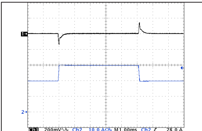
Figure 5: Output voltage response to step-change in load current (66 %-100 %-66 % of I_{out(max)} ; dI/dt = 0.1 A/\mu s ). Load cap: 1 \mu F ceramic and 15 \mu F tantalum capacitors. Ch 1: V_{out} (200 mV/div), Ch 2: I_{out} (10 A/div).
